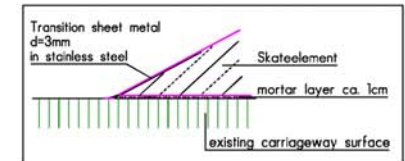
Transition sheet metal
