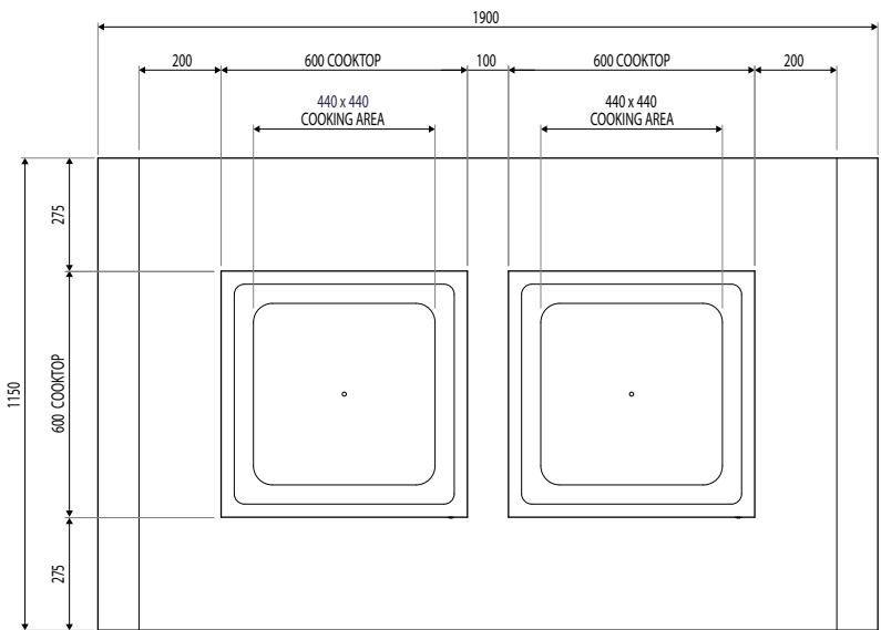
Rear View
